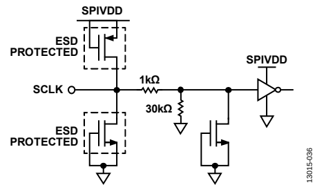
Figure 33. SCLK Inputs
