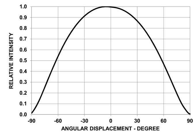
Figure 6: Radiation Pattern
