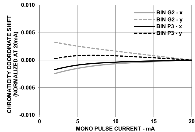
Figure 7: Chromaticity Coordinate Shift vs. Mono Pulse Current
