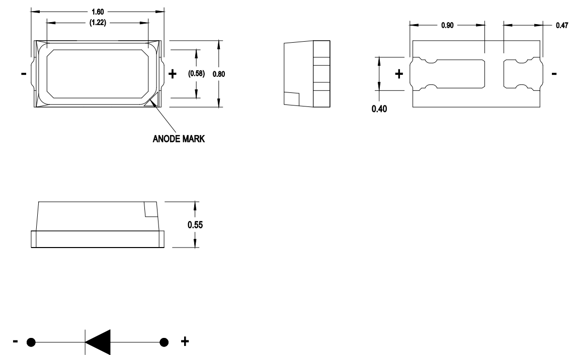
Figure 1: Package Drawing
