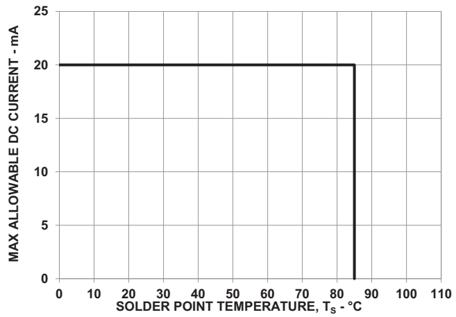
Figure 12: Maximum Forward Current vs. Solder Point Temperature. Derated based on T_{JMAX} = 95^{\circ}C , R_{\theta JS} = 80^{\circ}C/W
