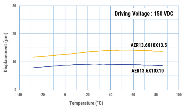
Figure 3 - Temperature vs. Displacement
