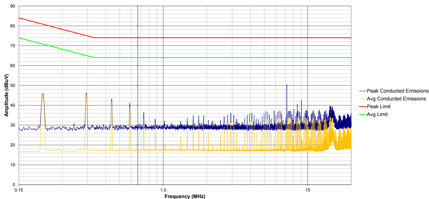
Figure 4.14. Si3404-Buck Non-Isolated EVB Conducted Emissions Measurements Results; 50 V Input, 5 V Output, 6.5 W Output Load
